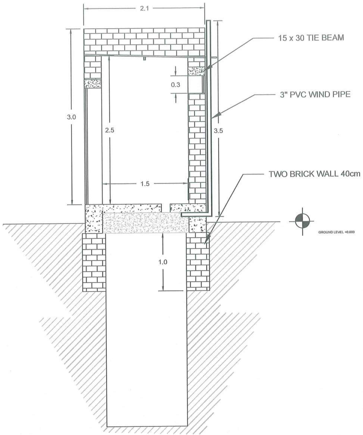
LATRINE SECTION A-A
